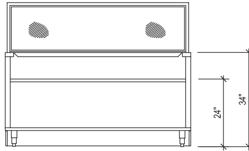
Elevation View ↑
